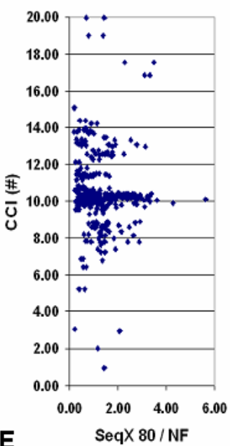
Amino Acid Co-locations vs. Charge Compatibility Index
