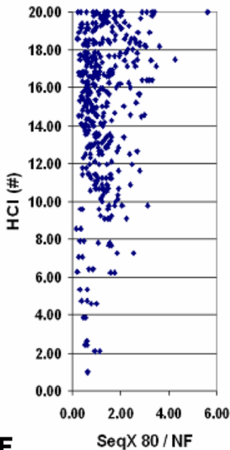
Amino Acid Co-locations vs. Hydrophobe Compatibility Index
