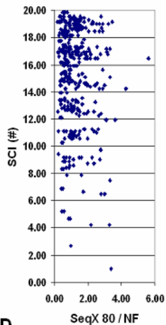
Amino Acid Co-locations vs. Size Compatibility Index
