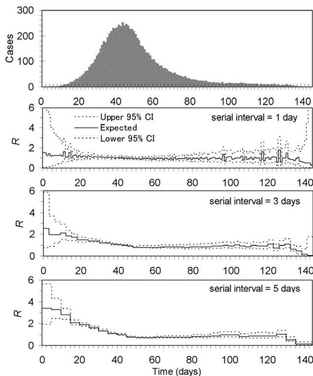
Figure 3 Epidemic curve and the corresponding effective reproduction numbers (R) with variable serial intervals. Time variation in the effective reproduction number (the number of secondary infections generated per case by generation) assuming three different serial intervals is shown. The serial interval was assumed to be 1 (second from the top), 3 (lower middle) and 5 days (bottom). Days are counted from September 9, 1918, onwards.
