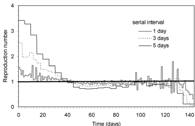
Figure 4 Comparison of the effective reproduction number assuming different serial intervals. Expected values of the effective reproduction number with a serial interval of 1 (grey), 3 (dashed black) and 5 days (solid black). The horizontal solid line represents the threshold value, R = 1 , below which the epidemic will decline to extinction. Days are counted from September 9, 1918, onwards.
